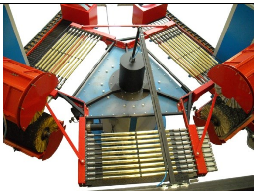
PIPE POLISHING MACHINE
