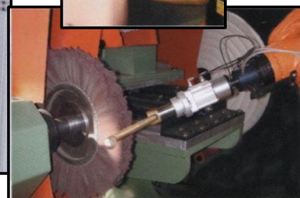
Station equipped with 2 robots for grinding working together or independently
