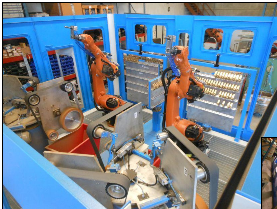
Station equipped with 2 robots for grinding working together or independently
